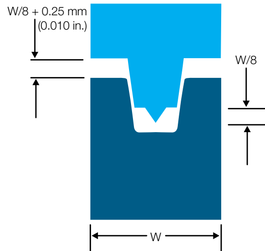
Figure 10.6 Shear joint
