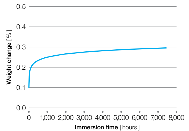
Figure 7.19 Water absorption of AvaSpire® AV-621 GF30 BG20
