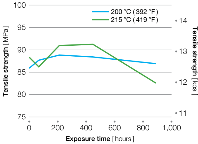
Figure 7.9 Tensile elongation of AV-621 NT after high-temperature aging
