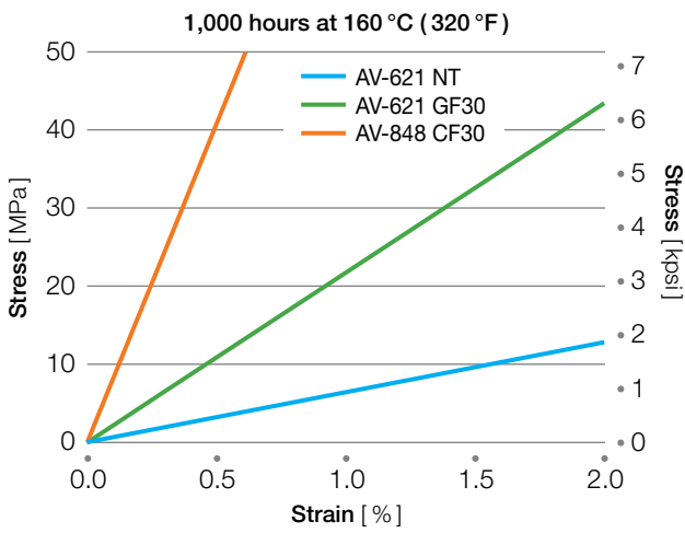
Figure 4.3 Isochronous curves at 160 °C (320 °F)
