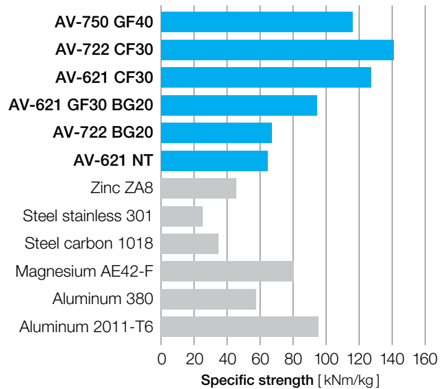
Figure 8.1 Specific strength comparison
