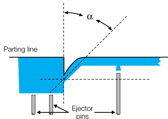
Figure 9.24 Tunnel gate
