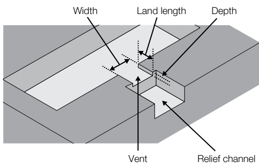
Figure 9.25 Vents
