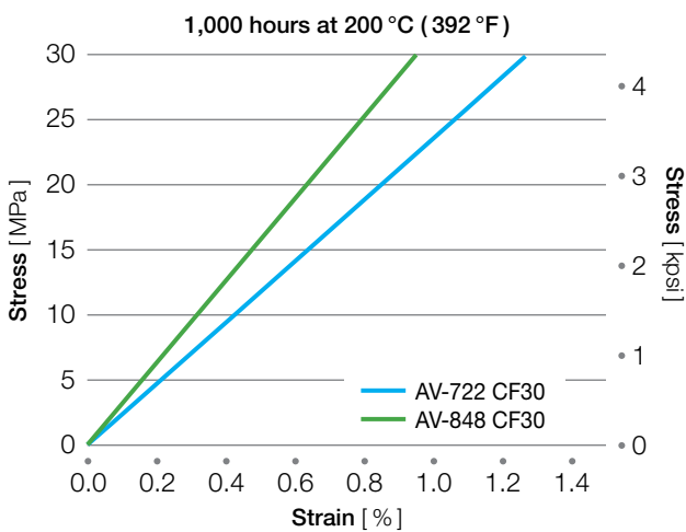
Figure 4.4 Isochronous curves at 200 °C (392 °F)
