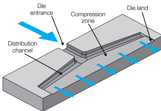
Figure 9.29 Coat hanger film die conceptual lower die plate
