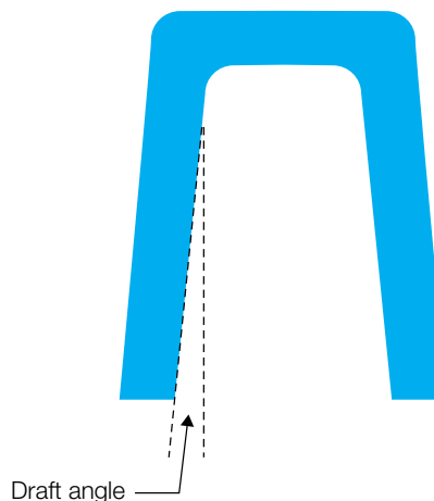
Figure 8.16 Draft – designing for mold release
