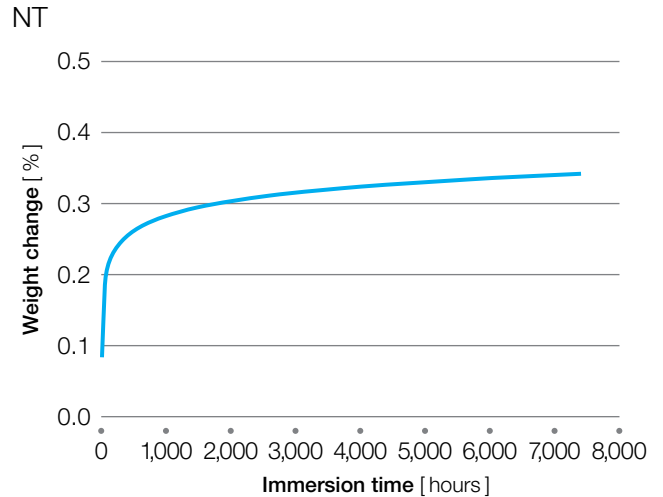
Figure 7.18 Water absorption of AvaSpire® AV-621
