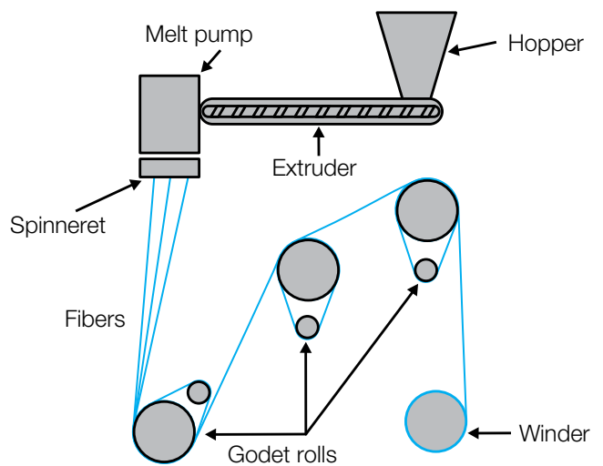
Figure 9.33 Fiber spinning process
