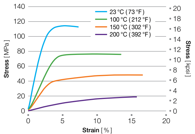
Figure 3.31 Stress-strain curves for AvaSpire® AV-722 BG20
