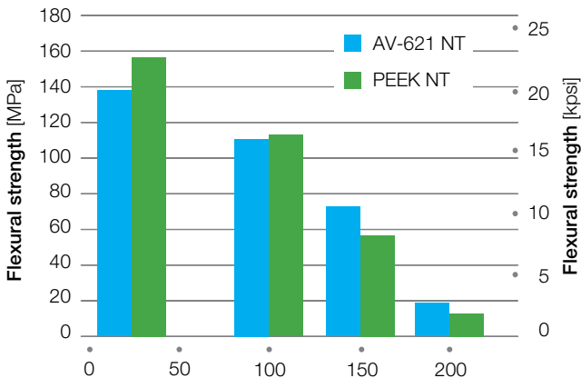
Figure 3.25 Flexural strength of AvaSpire® AV-621 NT and PEEK
