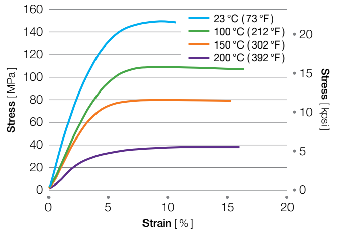
Figure 3.30 Stress-strain curves for AvaSpire® AV-621 CF30
